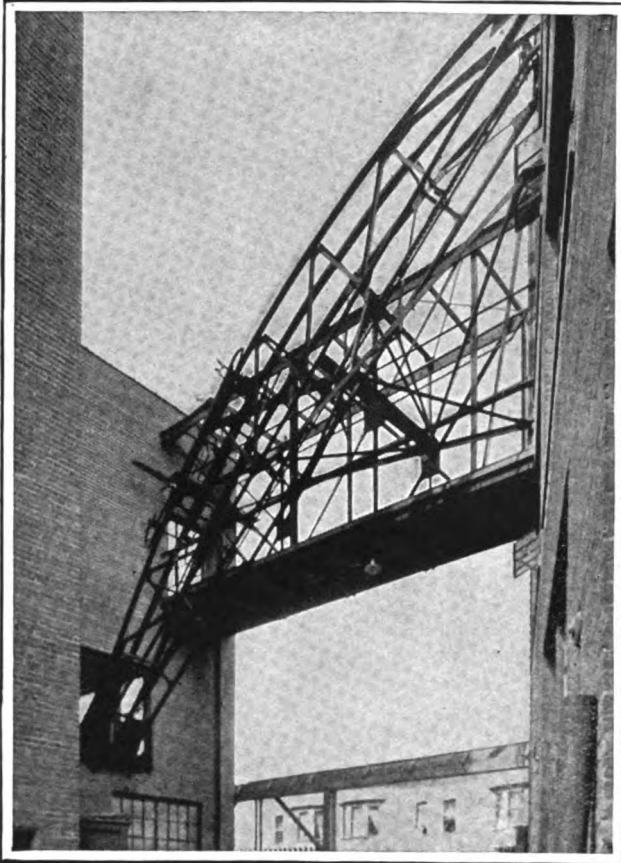
Fig. 29—In the Studebaker Corporation's factory in Detroit it is necessary to transfer automobile frames from one building to a floor two stories higher up in an adjacent building. For this purpose a conveyor system was installed by the Palmer-Bee Co. It consists of a structural steel frame with rails, over which the automobile frames are pulled by an endless chain conveyor
